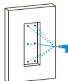
Take down the embedded box, then use a hand drill with 5mm diameter bit to make holes in the marked positions
