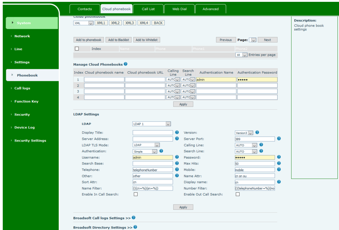
Picture 85- Web cloud phone book Settings
