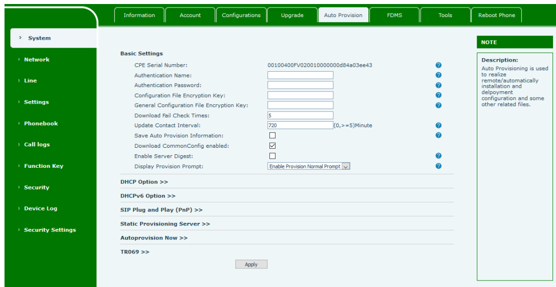
Picture 74- Page auto provision Settings
