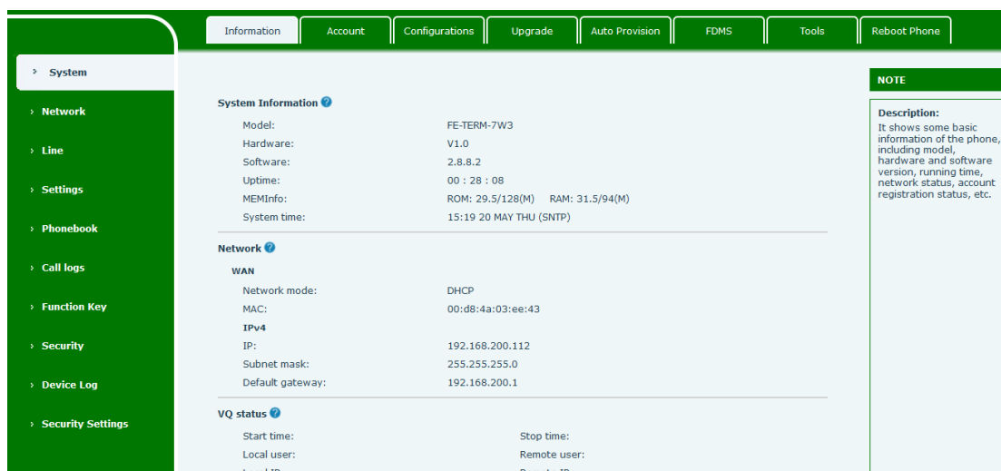
Picture 9- phone status
