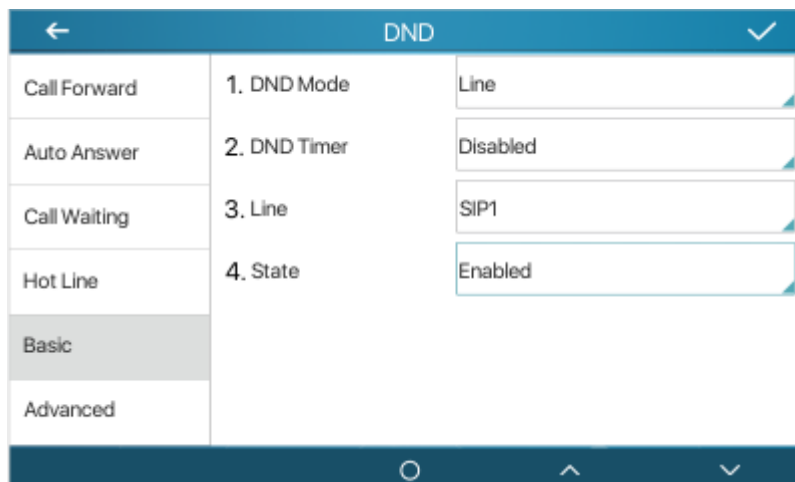
Picture 25- DND setting interface
