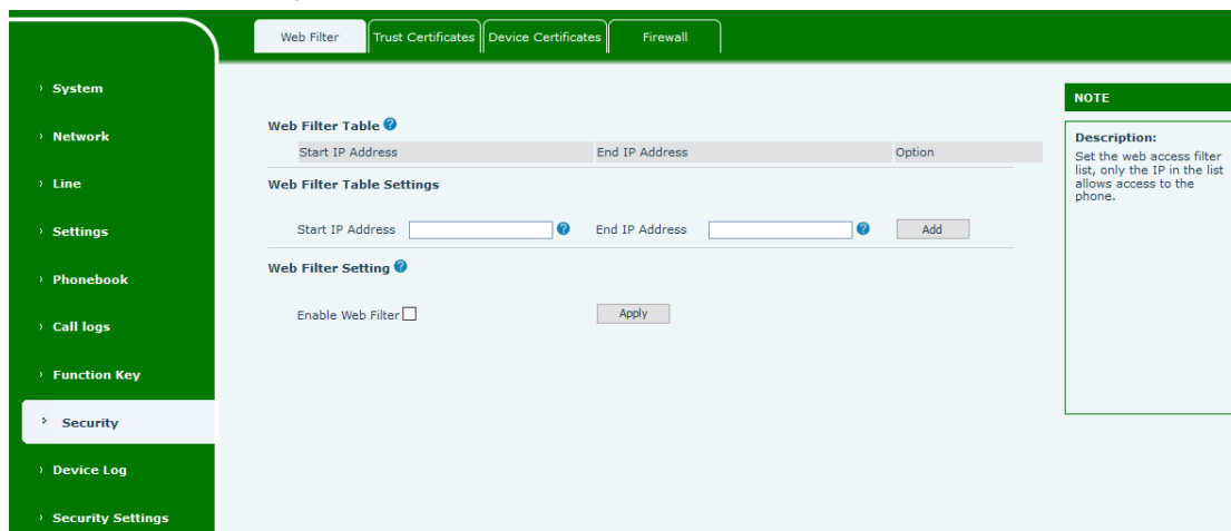
Picture 87- Web Filter settings
