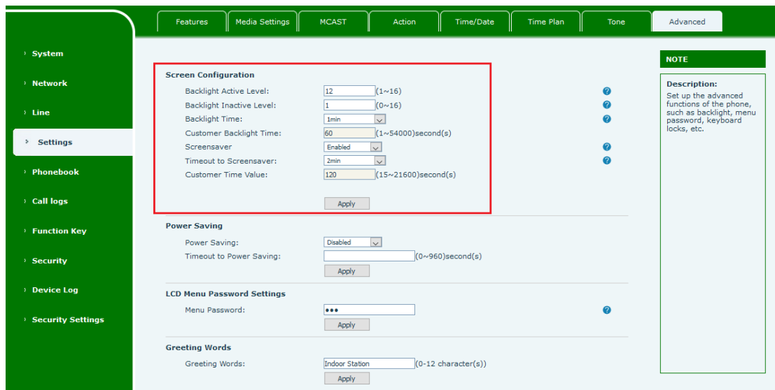
Picture 44 - set screen on webpage
