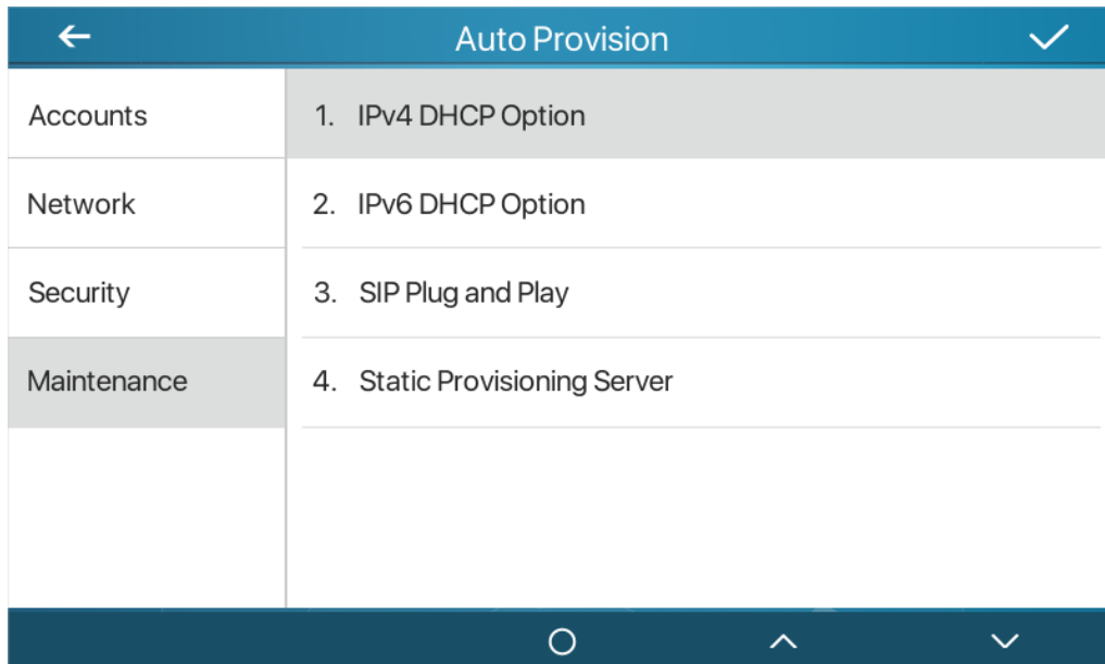
Picture 75- Phone auto provision settings
