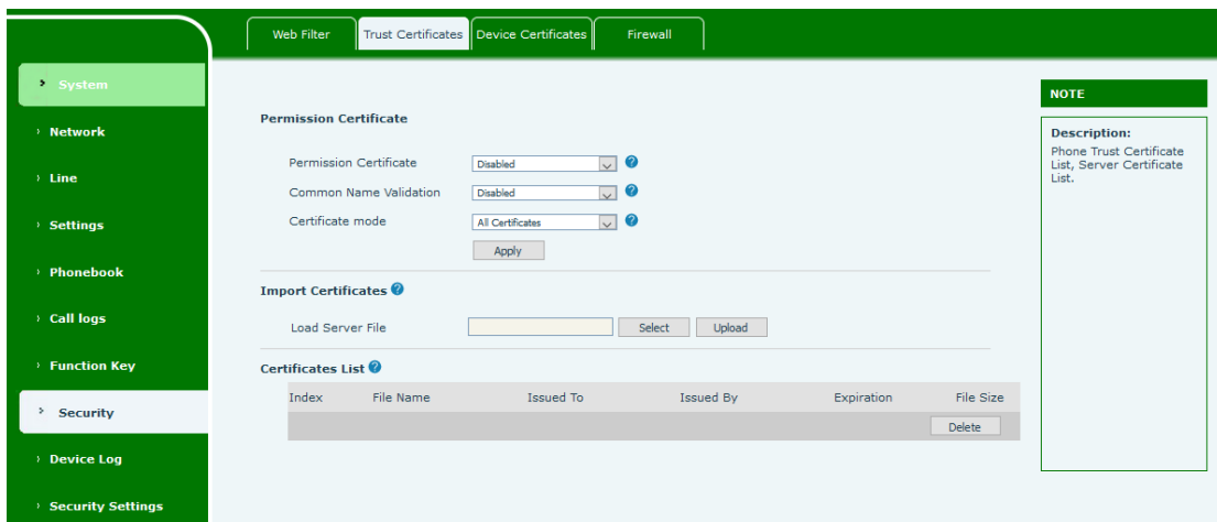
Picture 89- Certificate of settings
