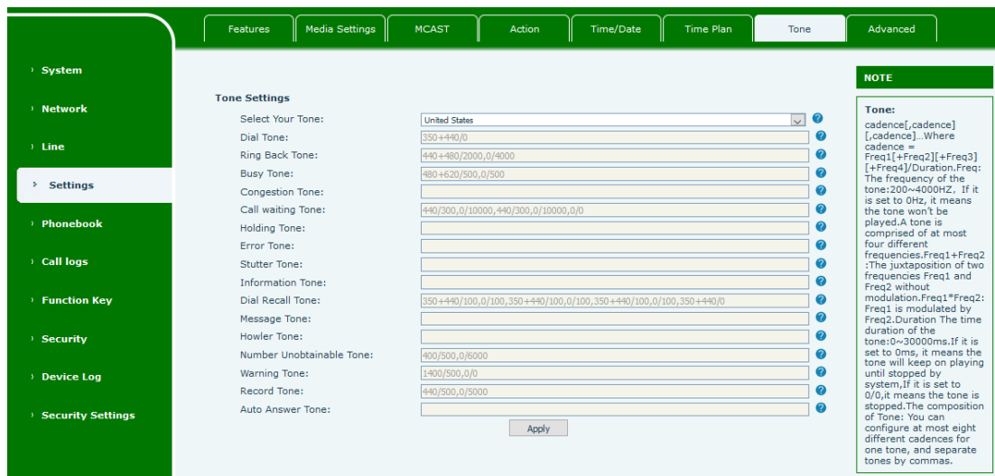
Picture 84- Webpage Tone
