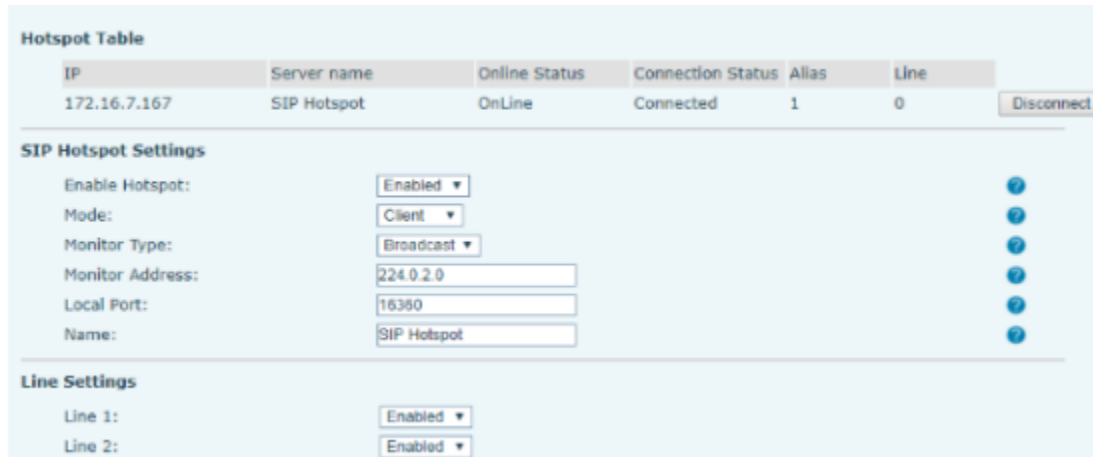
Picture 38- SIP hotspot client configuration
